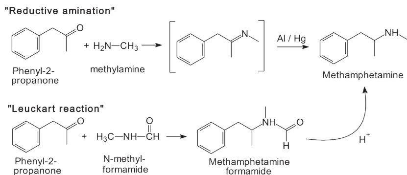
Fig. 7 Synthetic routes to methamphetamine from phenyl-2-propanone, a.k.a. phenylacetone. The "Reductive amination" route combines phenyl-2-propanone and methylamine to create an N-methylimine that undergoes reduction catalyzed by aluminum amalgam. The "Leuckart reaction" relies on nucleophilic attack of the phenyl-2-propanone carbonyl carbon by N-methylformamide to produce a methamphetamine formamide product that is converted by treatment with acid to methamphetamine. | Synthesewege zu Methamphetamine aus Phenyl-2-propanon, auch als Phenylacetone bekannt. Der Weg der „reduktiven Aminierung“ kombiniert Phenyl-2-propanon und Methylamin, um ein N-Methylimin zu erzeugen, das einer durch
